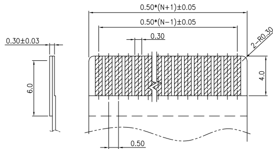
RECOMMENDED FPC/FFC DIMENSION
